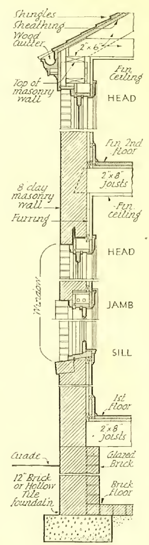
Wall Section
